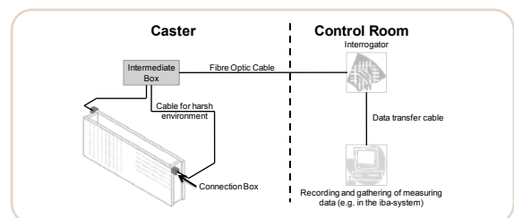
System Set-Up
