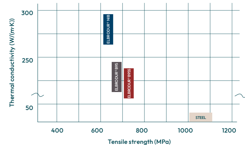
Thermal Conductivity and Strength of Copper Alloys
