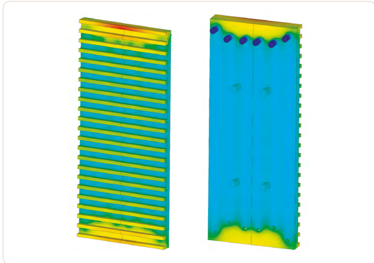
FEM calculation of the temperature distribution of copper staves under heat load.
