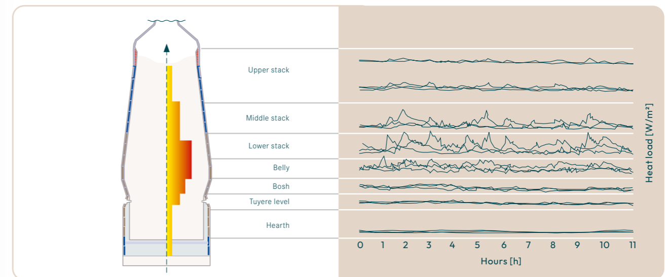
Typical heat load fluctuations in blast furnaces.
