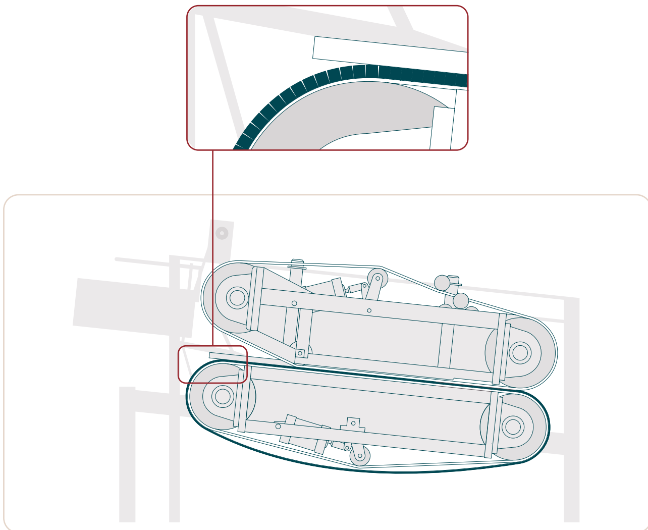
Continuous casting technology with dam blocks
