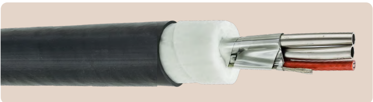
Pre-insulated Tube Bundle with Electric Tracer - 2 Core
